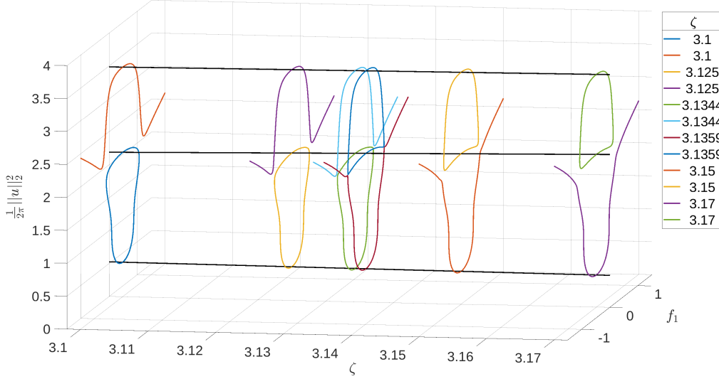
FIGURE 3. Same situation as in Figure 2. Zoom to the region close to the threshold where the continua change connectivity.
