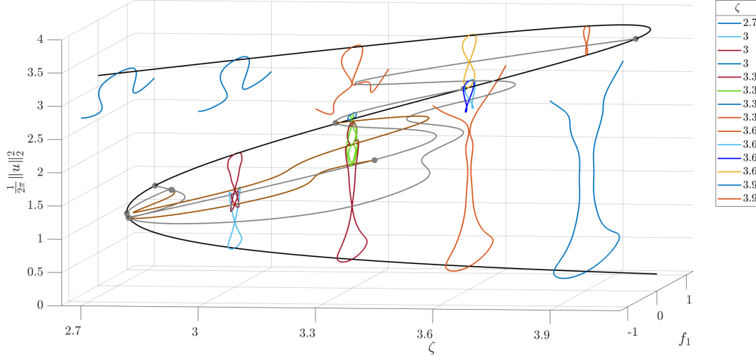
FIGURE 6. Continua of solutions (f_1, u) of (2) for selected values of the detuning \zeta . The other parameters were set to d = -0.1 , f_0 = 2 , k_1 = 1 , and \omega = 0 .
