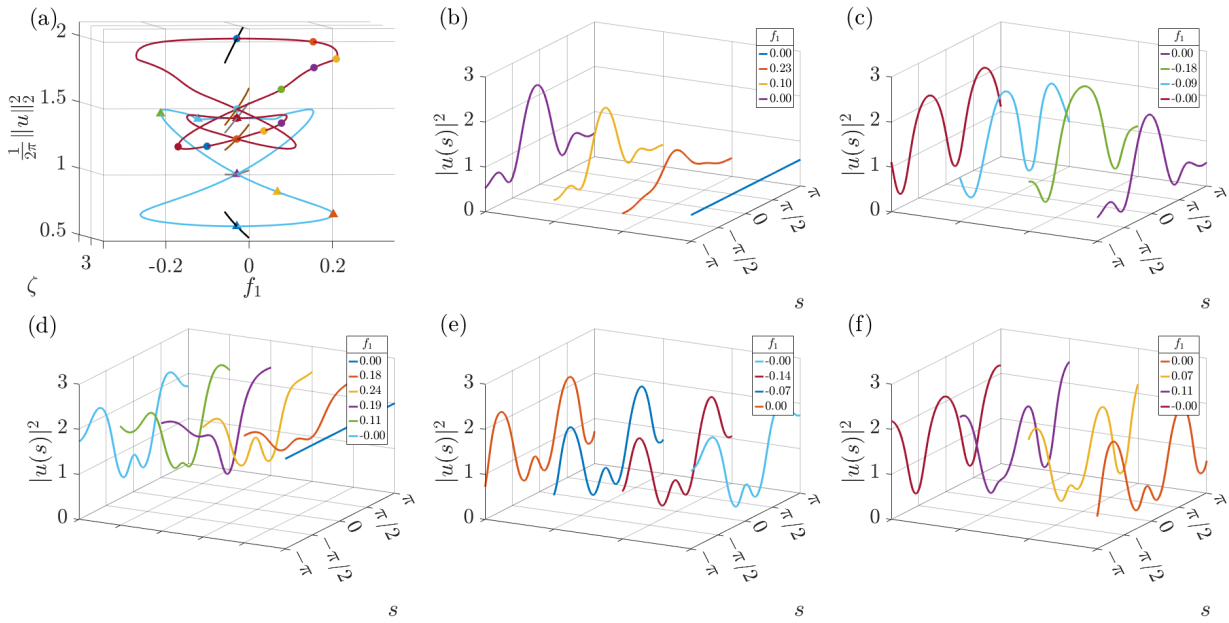
FIGURE 9. Zoom at \zeta = 3 and illustration of selected functions.
