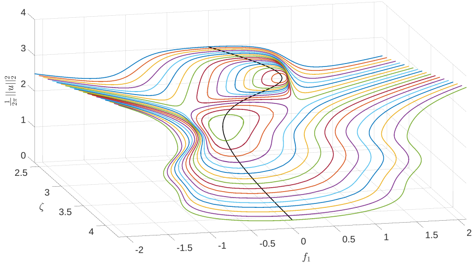
FIGURE 4. Same situation as in Figure 2, but depicted from a different angle and with more values of \zeta .
