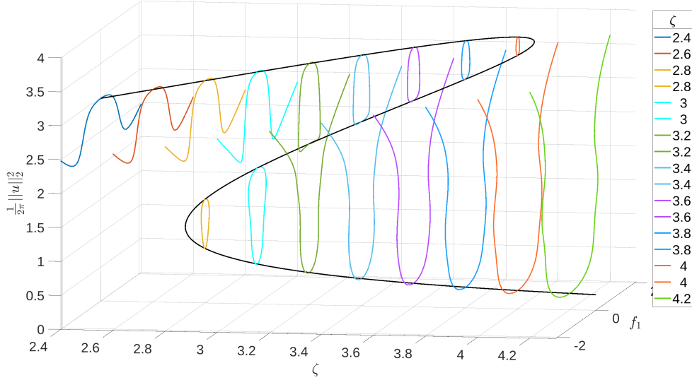
FIGURE 2. Continua of solutions (f_1, u) of (2) for selected values of the detuning \zeta . The other parameters were set to d = -0.1 , f_0 = 2 , k_1 = 1 , and \omega = 1 .
