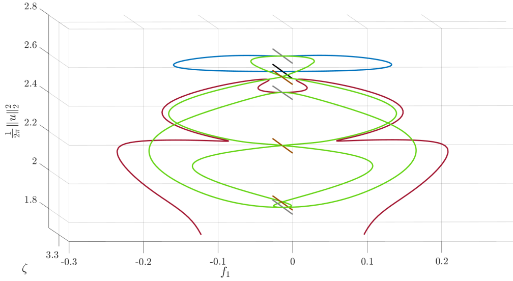
FIGURE 8. Zoom at \zeta = 3.3 .
