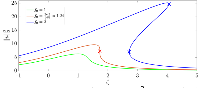
FIGURE 1. Curve of squared L^2 -norm of all constant solutions of (3) for f_1 = 0 and f_0 = 1 (green), f_0 = \frac{2\sqrt{2}}{\sqrt[4]{27}} \approx 1.24 (red) and f_0 = 2 (blue) when \zeta \in [-1, 5] . Turning points (if they exist) are marked with a cross.
