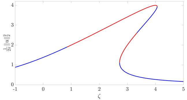
FIGURE 5. Sign of the second derivative of f_1 \mapsto \|u(f_1)\|_2^2 at f_1 = 0 ; blue=positive, red=negative.
