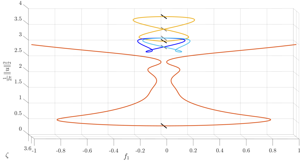
FIGURE 7. Zoom at \zeta = 3.6 .
