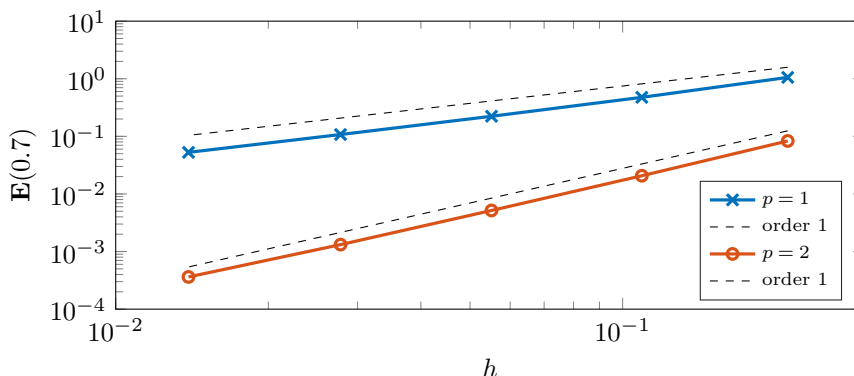
FIG. 1. Error from (6.1) at t = 0.7 for the test example.
