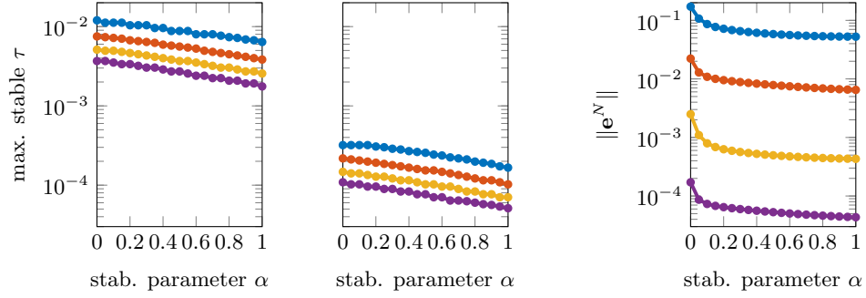
(A) Maximum stable time step \tau for the locally implicit method. (B) Maximum stable time step \tau for the Verlet method. (C) Error of the locally implicit scheme for time step size \tau = 5 \cdot 10^{-4} and final time t_N = T = 1 .
